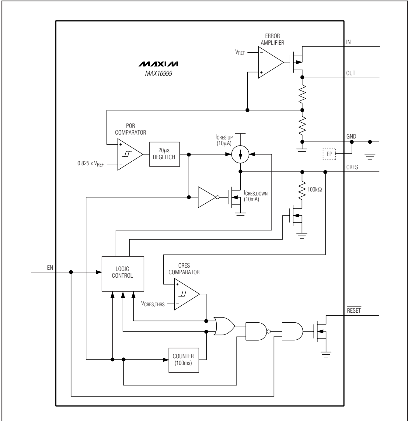
Figure 1. Block Diagram
